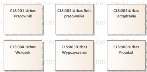
Figure I: Class Model
